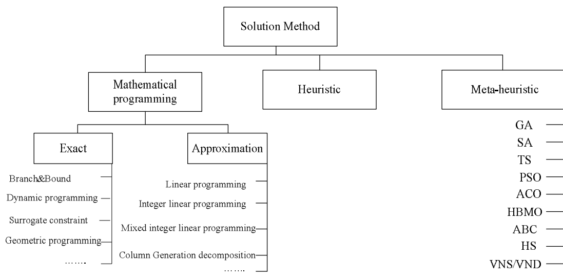
Fig. 3. RAP solution methods
