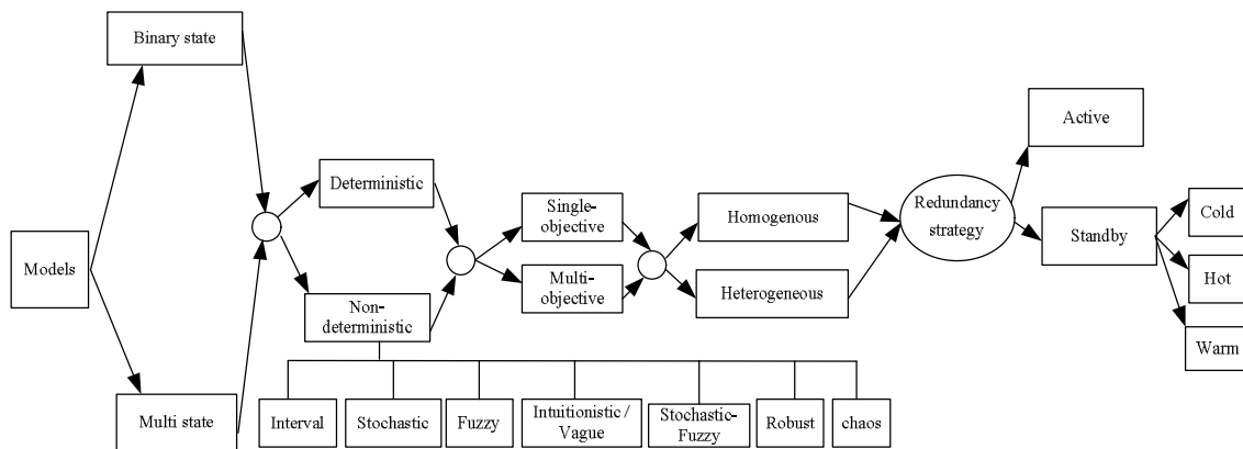
Fig. 2. RAP models
