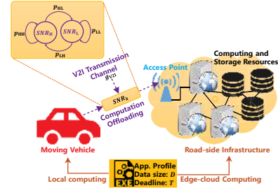
Fig. 1. Cooperative Vehicle-Infrastructure Computing Scenario.
