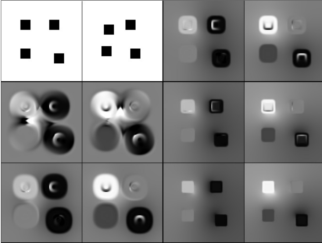
Figure 1: Computation of the optical flow for the square images with \alpha = 0.6 , s = 0.1 , and \eta = 0.95 . From top to bottom and from left to right we show the original image pair and the optical flow components (u, v) for \sigma_0 = 10 , \sigma_{12} = 5.7 , \sigma_{25} = 2.9 , \sigma_{37} = 1.4 , and \sigma_{50} = 0.8 .
