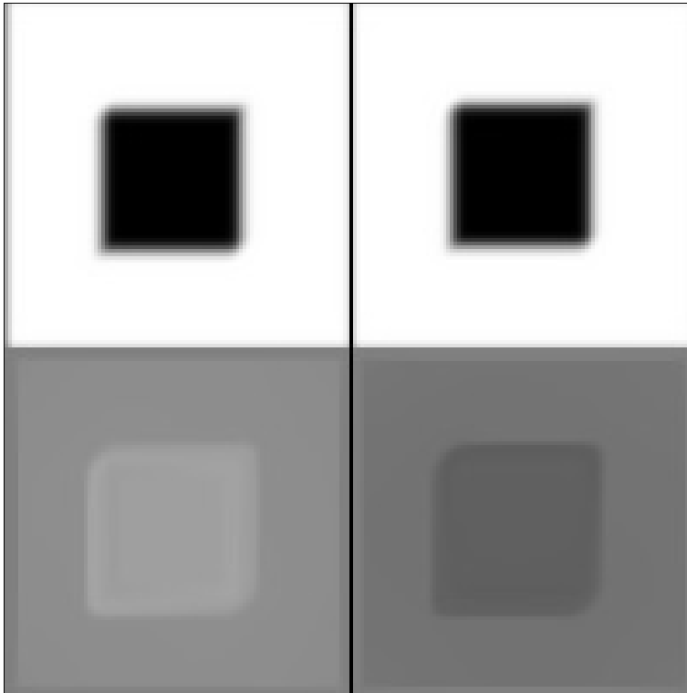
Figure 6: Computation of the optical flow for the Square2 sequence with \alpha = 0.6 , s = 0.1 , \sigma_0 = 10 , \sigma_n = 1 , and \eta = 0.95 .
