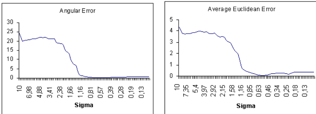
Figure 2: Left: Average angular error of the optic flow calculations for the squares in the first frame of Figure 1. Right: Corresponding average Euclidean error.
