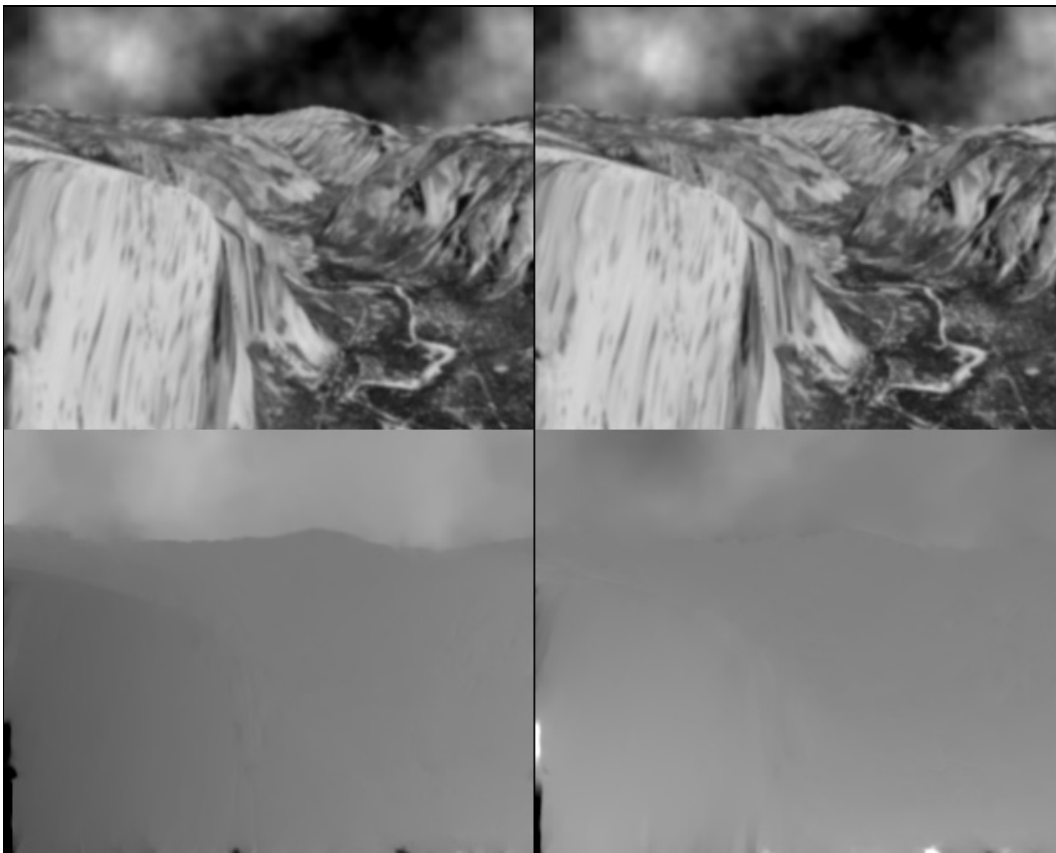
Figure 8: Computation of the optical flow for the Yosemite sequence with \alpha = 0.6 , s = 0.1 , \sigma_0 = 5 , \sigma_n = 1 , and \eta = 0.95 .
