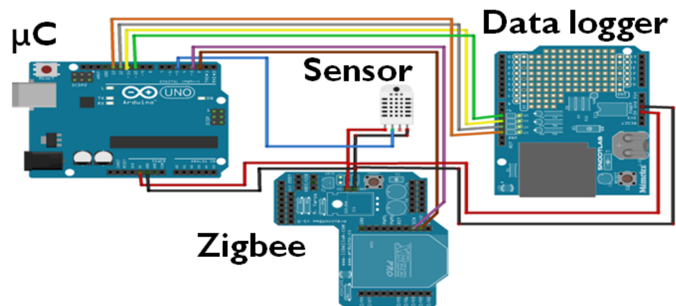
Figure 6. Environment sensing node annotated schematic diagram.
