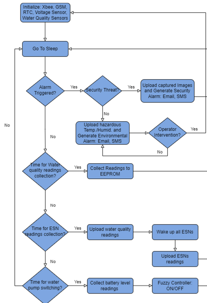
Figure 4. SCU flowchart.
