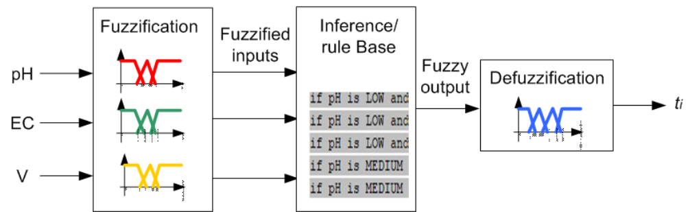
Figure 10. Fuzzy inference engine architecture.
