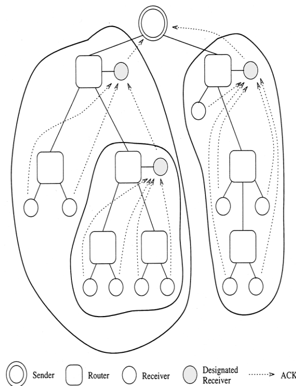
Fig 5: Multilevel Hierarchy of DR's.
