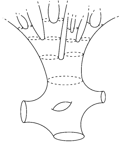
FIGURE 2. Cantor-tree endings made of hyperbolic cylinders.
