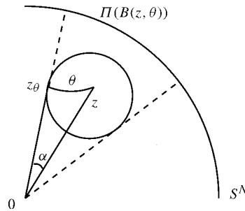
FIGURE 1. The setting of Lemma 1.
