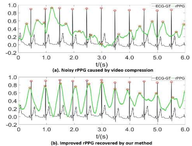
Figure 1. rPPG measurement from highly compressed videos. Due to video compression artifact and rPPG information loss, the rPPG in (a) has very noisy shape and inaccurate peak counts which lead to erroneous heart rate measures, while after video enhancement by STVEN, the rPPG in (b) shows more regular pulse shape with accurate peak locations comparing to the ground truth ECG.
