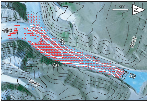
Fig. 16. Horizontal surface velocities on a glacier (name unpublished) at the northern slope of the Bhutan Himalaya towards the Tibet plateau ( 28.2^{\circ} N, 90.0^{\circ} E), derived from ASTER data of 20 January 2001 and 20 November 2001. Speed isolines are in m per year. Contour lines are in m a.s.l. and derived from the SRTM DTM. The dotted line at the calving front marks its position in 01/2001; the bold line is the 11/2001 position. Ice flux is an important factor influencing the development of proglacial ice-contact lakes.
