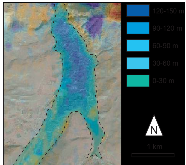
Fig. 12. Thickness of the 20 September 2002 avalanche deposits at Karmadon computed from ASTER DTMs of 22 July 2001 and 6 October 2002. The strong elevation changes to the upper right corner are due to errors in the ASTER DTMs in steep slopes (see also Figs. 4 and 5).
