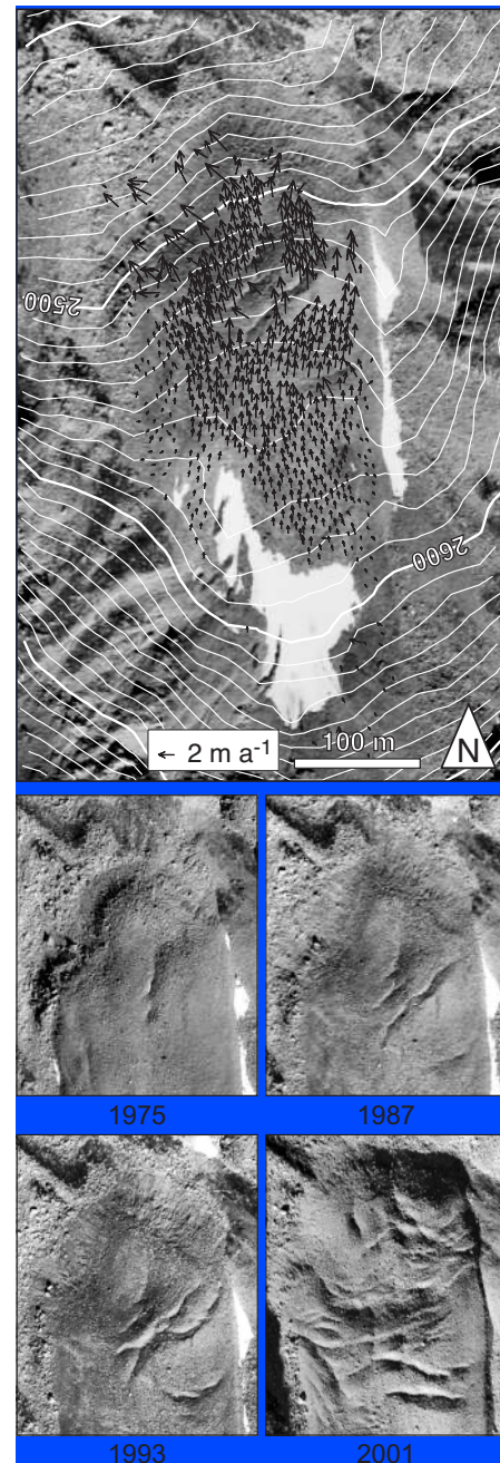
Fig. 14. Instability of a rockglacier terminus, Turtmanntal, Swiss Alps ( 46.2^{\circ} N, 7.7^{\circ} E). Upper panel: velocity vectors measured from airphotos of 1987 and 1993; lower panels: orthophotos of the terminus section of the rockglacier. Images of 1975, 1987, and 1993 are courtesy of swisstopo; the 2001 image is a linear array CCD (pushbroom) image taken by the HRSC-A camera, courtesy of Department of Geography, University of Bonn. The rockglacier instability led to enhanced rockfall and required construction of a protection dam (not depicted) (see also Roer et al., 2005).
