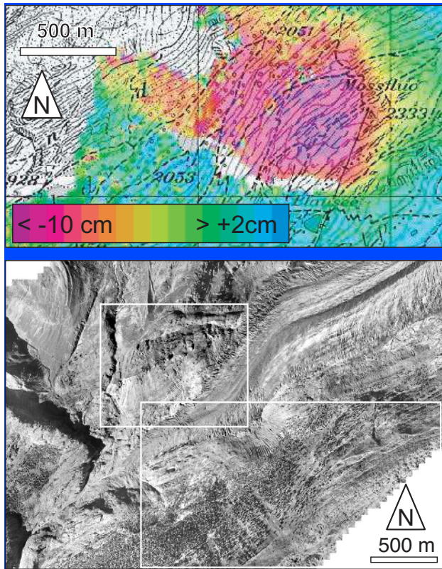
Fig. 19. Aletschwald, Swiss Alps ( 46.4^\circ\text{ N} , 8.0^\circ\text{ E} ). Upper panel: displacement magnitude map for a time interval of 1144 days (17 June 1993–4 August 1996) derived from repeat JERS SAR data. Displacement direction is assumed to be down-slope to the northwest. As yet the site has not been investigated in detail. However, a number of comparable movements situated nearby and studied already (see lower panel) hint to rock-slope creeping to be the cause for the displacements observed. Lower panel: Tongue of Aletsch Glacier with white rectangles indicating the location of this DInSAR study (lower rectangle) and the photogrammetric study Fig. 15 (upper rectangle).
