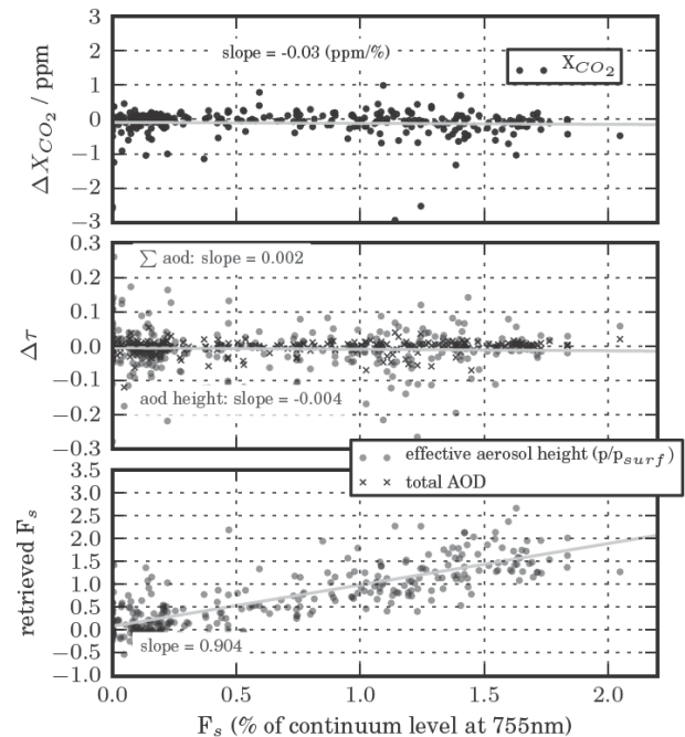
Fig. 8. Case #3b: Changes in retrieved X_{CO_2} as well as aerosol induced by chlorophyll fluorescence if fluorescence is fitted. Apart from the fluorescence fit, identical to case #3a, Fig. 5.
