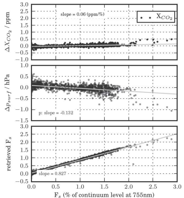
Fig. 6. Case #1b: Changes in retrieved X_{CO_2} induced by chlorophyll fluorescence if fluorescence is fitted. Both simulation and retrieval use a Rayleigh-only atmosphere.
