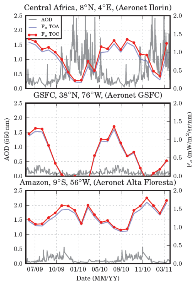
Fig. 13. Temporal series of top-of-atmosphere (TOA) fluorescence and the subsequent top-of-canopy (TOC) fluorescence after compensation of atmospheric extinction (scattering + absorption) for locations in Central Africa (top), Greenbelt, MD (middle) and the Amazon (bottom).
