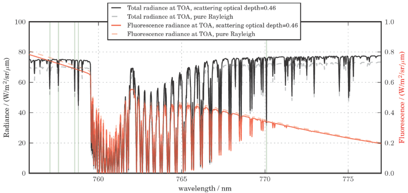
Fig. 2. Simulated noise-free spectrum with GOSAT spectral resolution. Solar zenith angle = 26.35°; surface albedo \approx 0.2 ; aerosol + cloud optical depth = 0.46. The fluorescence spectrum at the TOA is modeled once in a pure Rayleigh atmosphere and once including aerosol and cloud scattering of the emission emanating from the surface. Positions of Fraunhofer lines most suitable for fluorescence retrievals in the GOSAT spectral range are indicated by green lines.
