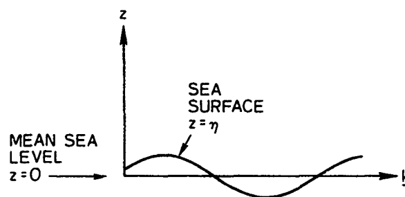
Fig. 2.2. SEA SURFACE IN THE PLANE OF WAVE PROPAGATION.
