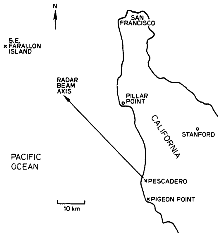
Fig. 8.1. LOCATIONS OF ANEMOMETERS. These are indicated by x at the Farallons, Pescadero, and Pigeon Point.
