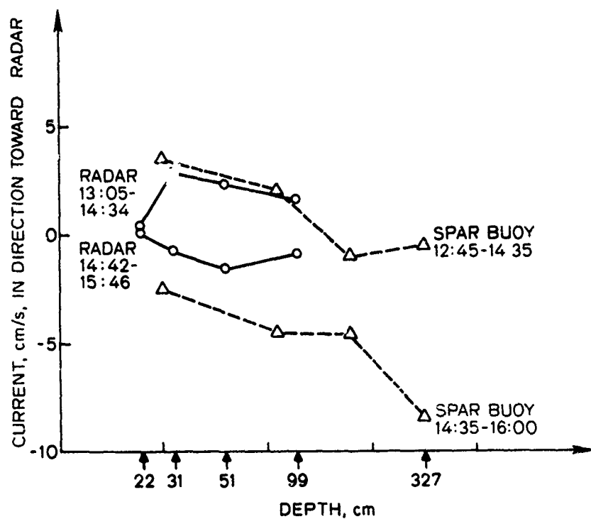
Fig. 7.1. COMPARISON OF RADAR-INFERRED DRIFT AND SPAR-BUOY DRIFT (CLUSTER 2) OBTAINED ON 19 JANUARY 1978. Horizontal axis is logarithmic in depth, and a logarithmic profile is assumed. The approaching Bragg line was used.
