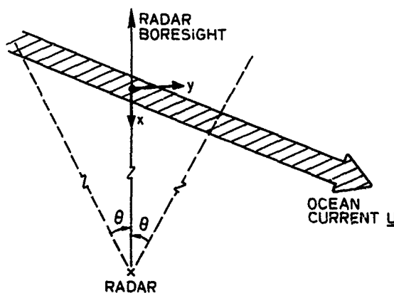
Fig. 8.3. BACKSCATTER GEOMETRY.
