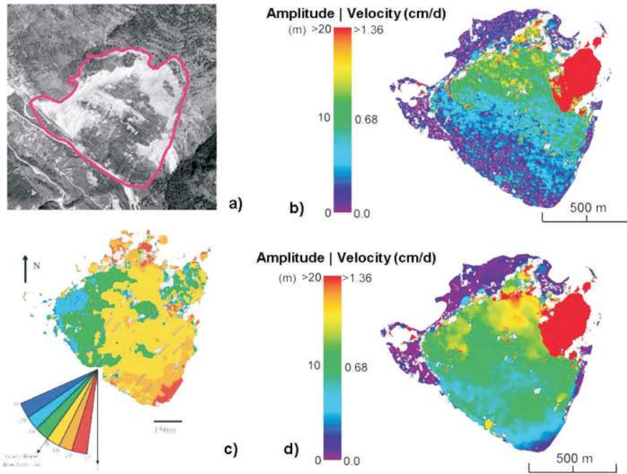
FIG. 4. – Displacement and velocity maps calculated using aerial image correlation (1995 – 1999) of “La Clapière” landslide. a) Aerial orthophotograph of the landslide. b) Horizontal velocity. c) Orientation displacement map in the horizontal plan. d) Vertical velocity map.
