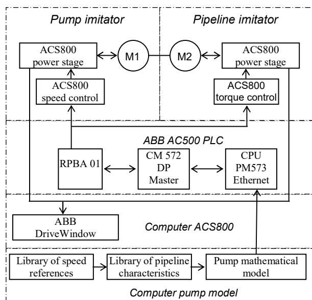
Fig. 2 HIL simulator of a pumping station
