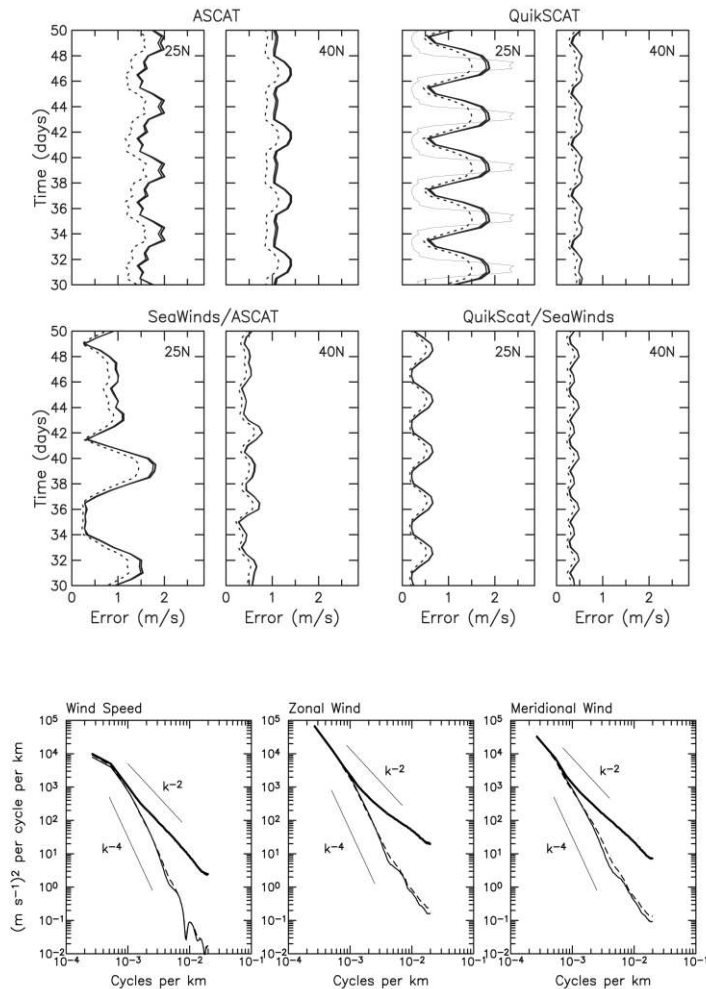
Figure 2. Upper panels: Time series of the RMS mapping errors of meridional (solid lines) and zonal (dotted lines) wind estimates constructed at latitudes of 25°N and 40°N from various combinations of scatterometer observations with 2° by 2° by 4-day smoothing. The three solid lines correspond to different assumed forms for the spatial autocorrelation function; the small differences show that the results are not strongly sensitive to the details of the spatial autocorrelation function; the most limiting factor for construction of wind fields is the short decorrelation time scale of the surface wind field. (The thin solid line in the QuikSCAT panel is a time series of the RMS (Root-Mean-Square) mapping errors at 25°N with 2° by 2° by 1.5-day smoothing.) (From [97].) Lower panels: Along-track wavenumber spectra of wind speed and the zonal and meridional wind components in the eastern North Pacific, accumulated over 2004, computed from QuikSCAT observations (heavy solid lines), NCEP (National Centers for Environmental Prediction) analyses (thin solid lines) and ECMWF analyses (dashed lines; the 2004 version had ~40km grid spacing compared to the current ~25km). Note the drop-off of spectral energy in the two operational forecast models at wavelengths shorter than about 1000 km (wavenumbers higher than about 10 -3 cycles per km). (From [20].)
