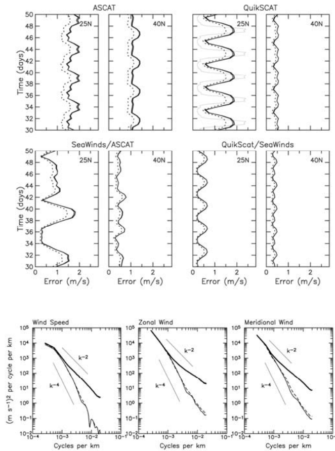
Figure 2. Upper panels: Time series of the RMS mapping errors of meridional (solid lines) and zonal (dotted lines) wind estimates constructed at latitudes of 25°N and 40°N from various combinations of scatterometer observations with 2° by 2° by 4-day smoothing. The three solid lines correspond to different assumed forms for the spatial autocorrelation function. The small differences show that the results are not strongly sensitive to the details of the spatial autocorrelation function; the most limiting factor for construction of wind fields is the short decorrelation time scale of the surface wind field. (The thin solid line in the QuikSCAT panel is a time series of the RMS mapping errors at 25°N with 2° by 2° by 1.5-day smoothing.) (From [97].) Lower panels: Along-track wavenumber spectra of wind speed and the zonal and meridional wind components in the eastern North Pacific, accumulated over 2004, computed from QuikSCAT observations (heavy solid lines), NCEP analyses (thin solid lines) and ECMWF analyses (dashed lines; the 2004 version had \sim 40 km grid spacing compared to the current \sim 25 km). Note the dropoff of spectral energy in the two operational forecast models at wavelengths shorter than about 1000 km (wavenumbers higher than about 10^{-3} cycles per km). (From [20].)
