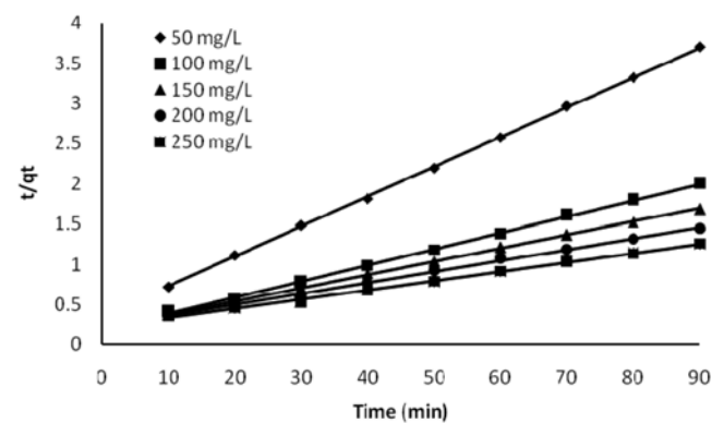
Fig. 7. Pseudo-second-order reaction for MB adsorbed onto CNSAC at different concentrations (MB concentrations=50-250 mg/L, adsorbent dose=2 g/L, volume of sample=100 mL and equilibrium time=90 min).
