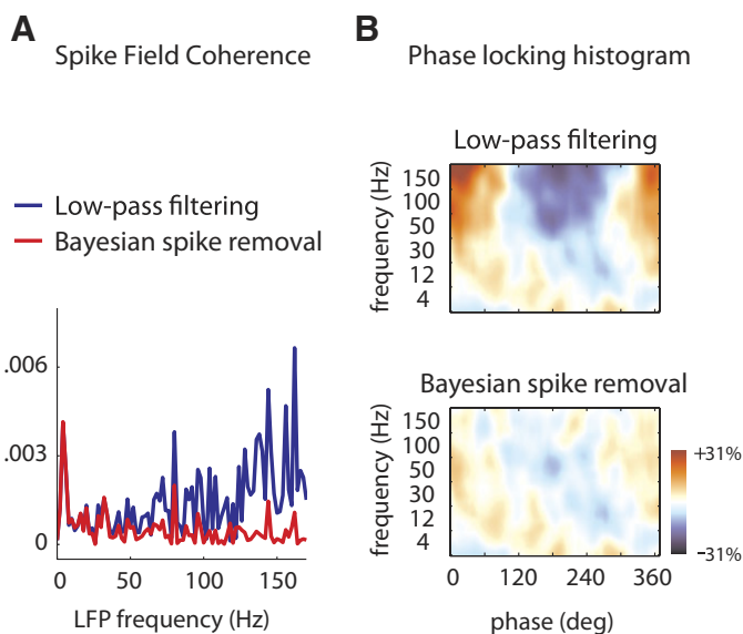
FIG. 9. Phase-locking analysis results for an illustrative MT neuron. A: SFC of the LFP signal before (blue trace) and after (red trace) spike removal. B: phase-locking histogram before (top panel) and after (bottom panel) spike removal.
