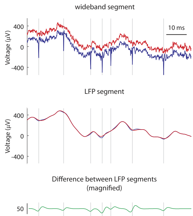
FIG. 3. Composite wideband and LFP signal segments with and without spike waveforms. Segment of a spike-free, phase-randomized wideband signal (top panel) before (red line) and after (blue line) the addition of spike waveforms. Filtered versions of these signals (middle panel) and their difference (bottom panel) reveal the effect of the addition of spike waveforms on the LFP component of the composite signal.
