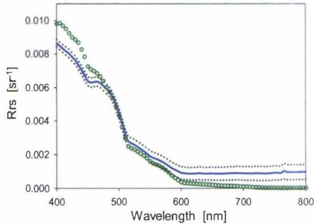
Fig. 6. Average R_{rs} (solid blue) and the one standard deviation (dotted lines), calculated using Eq. (4b). Green line is modeled R_{rs} with Chl = 0.05 mg m -3 using the Morci-Maritorena bio-optical model [16].
