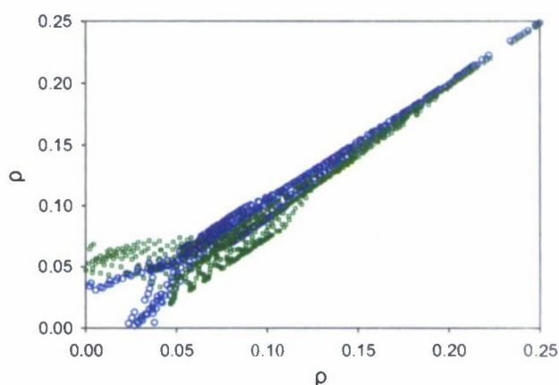
Fig. 5. Scatter plot between \rho(\text{Chl} = 0.05) and \rho(\text{Chl} = 0.025) , blue symbol; and between \rho(\text{Chl} = 0.05) and \rho(\text{Chl} = 0.1) , green symbol.
