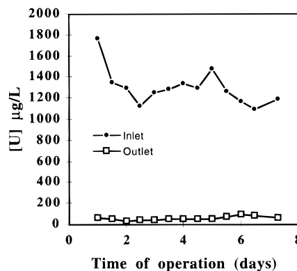
FIGURE 7. Pilot rhizofiltration system performance at the high level of U concentrations in influent. The influent was spiked for 1 week with UO 2 (C 2 H 3 O 2 ) 2 stock solution (350 mg U/L) to bring the concentration over 1000 µg/L at a flow rate of 1.05 L/min.
