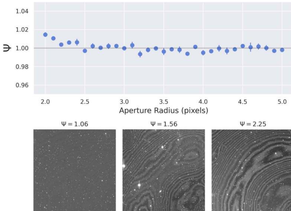
Figure 5. The Uniform Background Indicator is \Psi \approx 1 for a range of aperture sizes on images of Gaussian noise (top). This validates interpreting \Psi \approx 1 as measuring no correlated background noise in an image. Three example i -band images and their \Psi values are shown (bottom). More prominent atmospheric fringes correlates with an increase in the value of \Psi .
