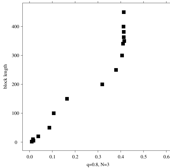
Fig. 12. Effective Rényi transfer entropy T_{0.8:SP\&500 \rightarrow DAX}^{(R)}(m, m) for a 3-letter alphabet as a function of the block length m . DAX and SP&500 min prices are employed. The correlation time is between 200–300 minutes.
