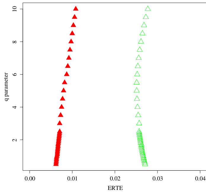
Fig. 13. The ERTE as a function of q . The alphabet size is set to N = 3 . DAX and SP&500 min prices are employed. The red curve corresponds to T_{q;SP\&500 \rightarrow DAX}^{(R,eff)}(m, m) while the green curve denotes T_{q;DAX \rightarrow SP\&500}^{(R,eff)}(m, m) . (For interpretation of the references to colour in this figure legend, the reader is referred to the web version of this article.)
