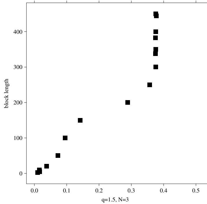
Fig. 11. Effective Rényi transfer entropy T_{1.5:SP\&500 \rightarrow DAX}^{(R)}(m, m) for a 3-letter alphabet as a function of the block length m . DAX and SP&500 min prices are employed. The correlation time is between 200–300 minutes.
