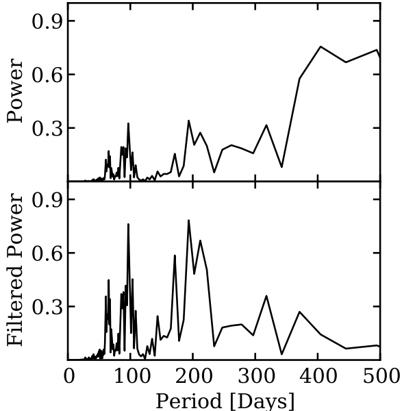
FIG. 7.— Normalized power spectrum of \dot{\nu} for 1E 1048.1–5937 over 12 years. The top panel is red-noise unfiltered, and the bottom panel has been passed through a high-pass filter. See Section 3 for details.
