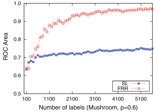
(a) p = 0.6, \#examples = 100 , for FRR
