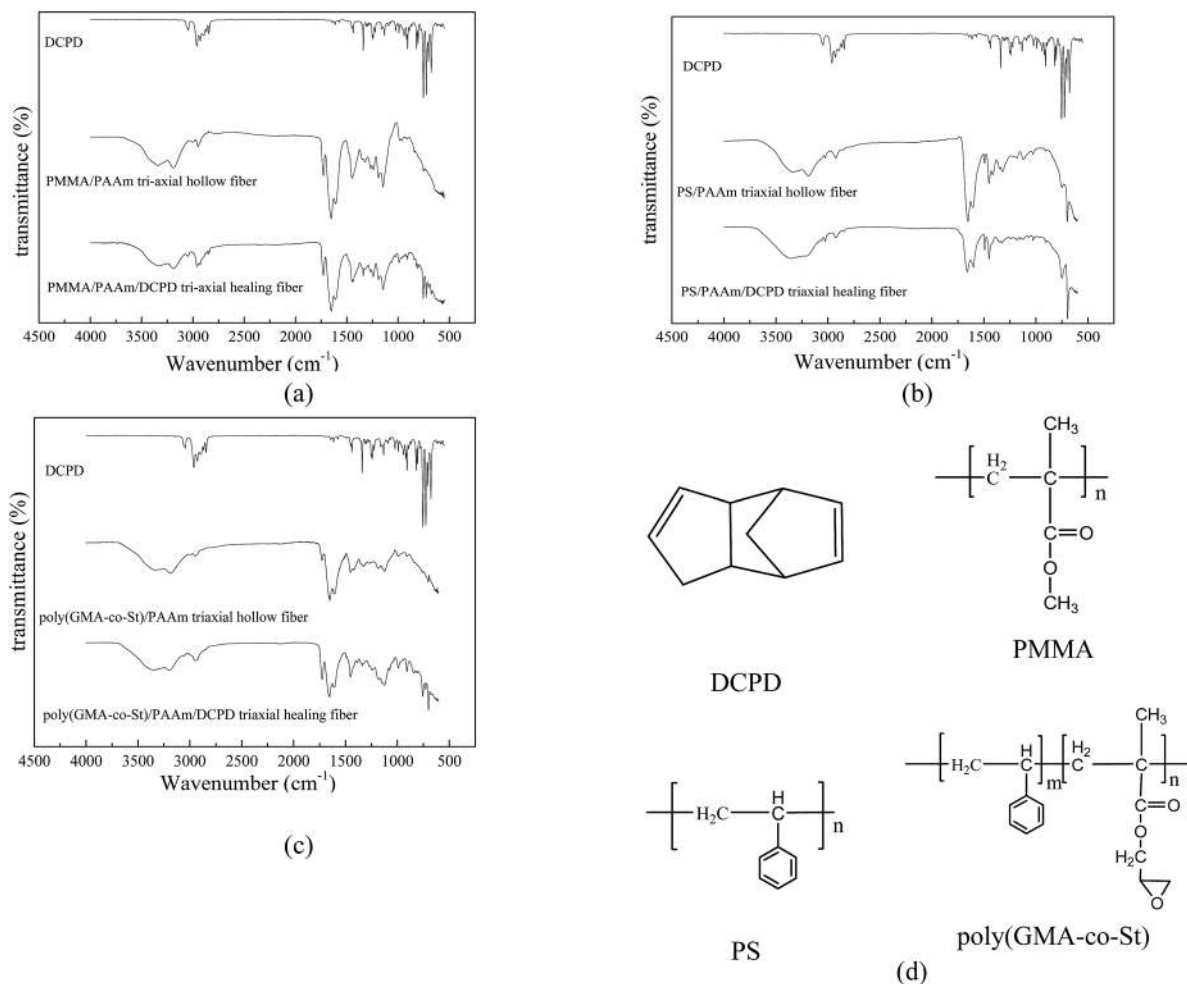
Fig. 7 FTIR spectra of (a) DCPD, PMMA/PAAm tri-axial hollow fiber and PMMA/PAAm/DCPD tri-axial fiber, (b) DCPD, PS/PAAm tri-axial hollow fiber and PS/PAAm/DCPD tri-axial fiber, (c) DCPD, poly(St-co-GMA)/PAAm tri-axial hollow fiber and poly(St-co-GMA)/PAAm/DCPD tri-axial fiber. (d) The chemical structure of polymers and DCPD.
