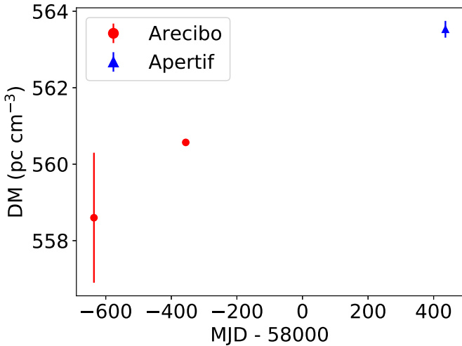
Fig. 3. Structure-optimised DM of R1 at 1400 MHz as measured at different epochs. The two Arcetibo data points are from Scholz et al. (2016) and Hessels et al. (2019) , respectively. For Apertif, we averaged the DM of the four bursts for which we determined a structure-optimised DM. The error bars indicate 1\sigma uncertainties. The uncertainty on the second data point is smaller than the circle. The DM has significantly increased from 560.57(7) pc cm ^{-3} in September 2016 to 563.5(2) in November 2018.
