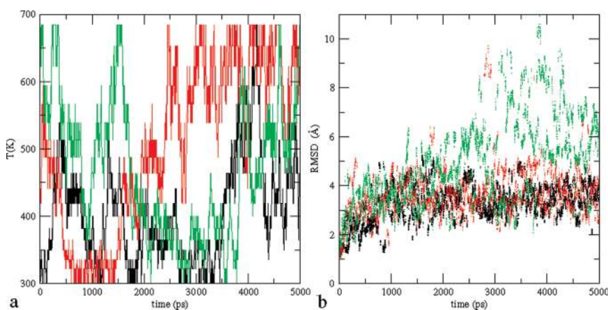
Figure 3. (a) Temperature trajectories for three representative replicas with the effective temperature of the protein initially at low ( T = 310 K), intermediate ( T = 419 K), and high ( T = 684 K) temperatures for the \beta -hairpin system. (b) The protein heavy atom rmsd versus time at each of the above temperatures when replicas visit those temperatures (black, T = 310 K; red, T = 419 K; green, T = 684 K).
