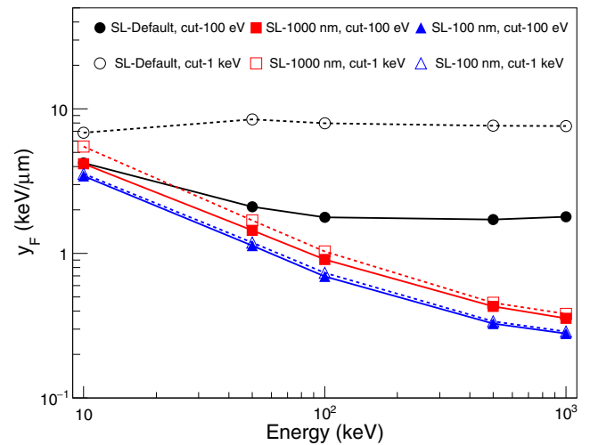
FIG. 10. Frequency-mean lineal energy as a function of the incident electron energy, using two different values for the tracking cut 100 eV and 1 keV. SL is the step-size limit. SL was set equal to 1 mm (default value for this test), 1 \mu\text{m} and 100 nm. Error bars are not included since they are smaller than the symbols. The plot demonstrates that SL should be substantially less than the size of scoring volume. [Color figure can be viewed at wileyonlinelibrary.com ]
