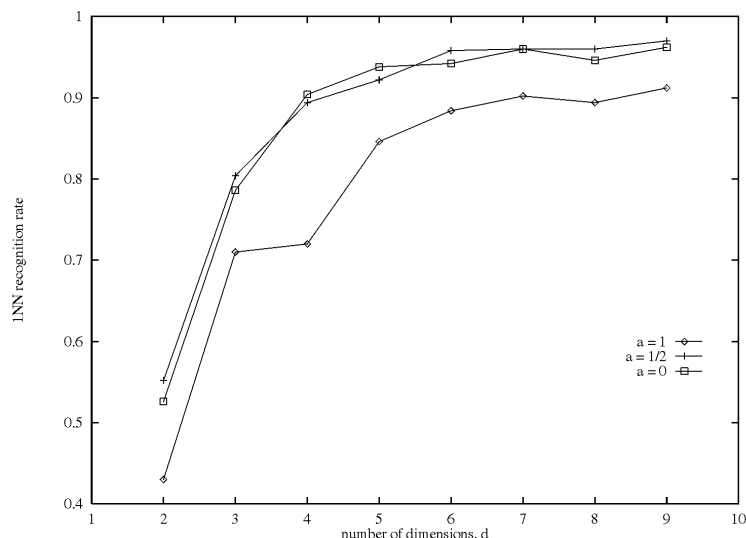
Fig. 8. Plot of 1NN recognition accuracy vs. number of dimensions.
