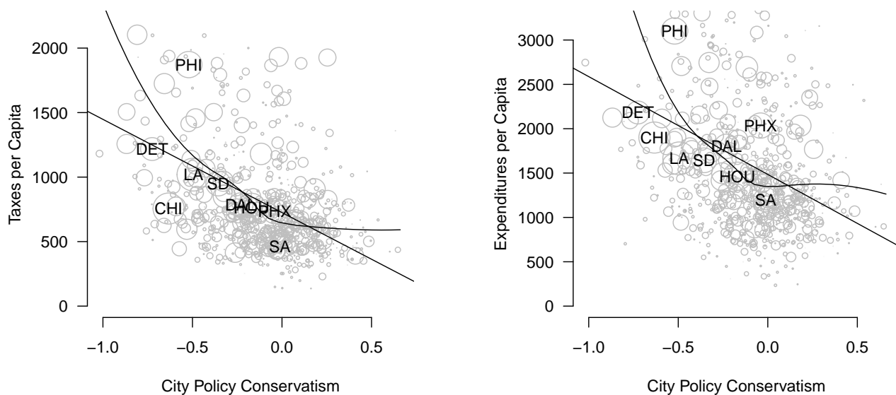
Figure 3: Responsiveness- Zoomed. This Figure repeats the panels on the right side of Figure 2 with a restricted y-axis. A linear regression line and loess curve is shown in each panel.
