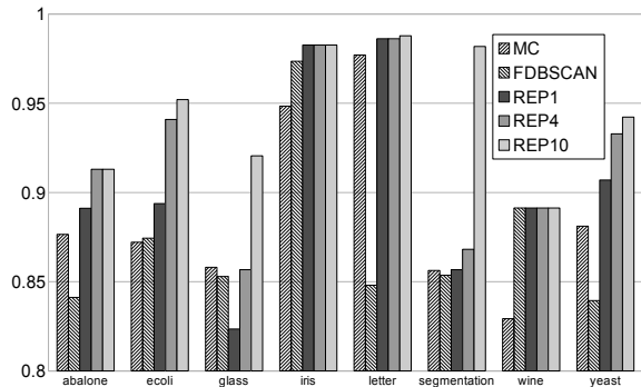
Figure 5: ARI on all datasets.
