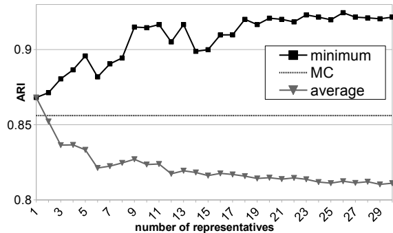
Figure 6: ARI vs. the number of representatives.
