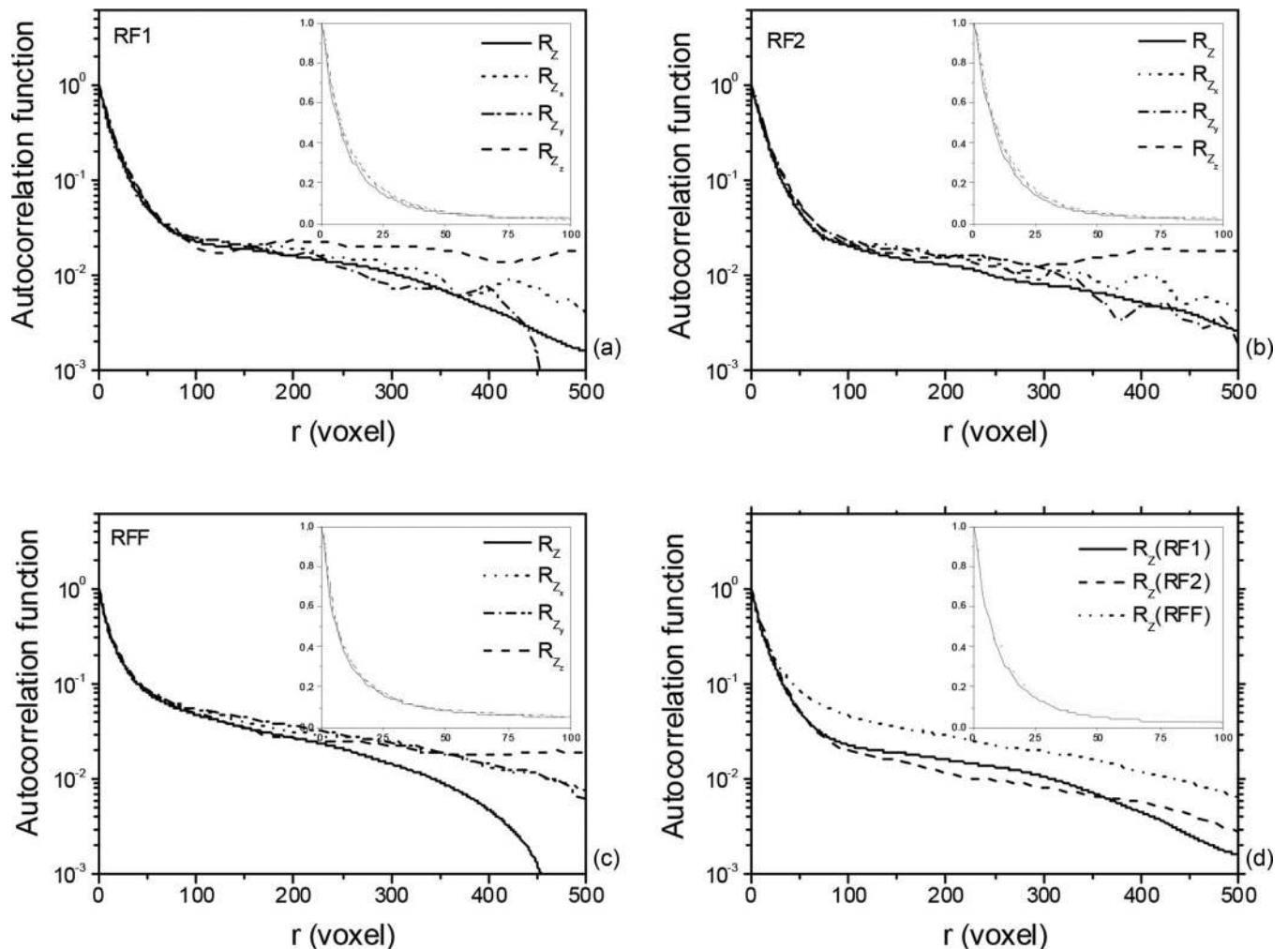
FIG. 5. Autocorrelation functions ( R_{Zx} , R_{Zy} , and R_{Zz} ) and the average value R_Z for a RF1 sample (a), a RF2 sample (b), and a RFF sample (c).
