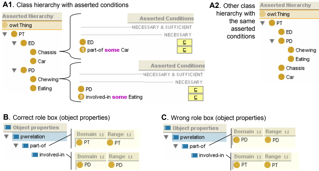
Fig. 5. Two class hierarchies and two role (object property) hierarchies in Protégé.
