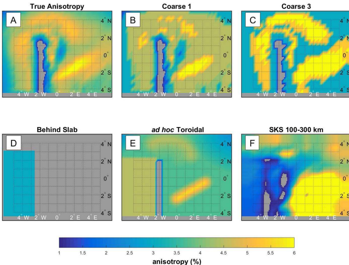
Figure 11. Distribution of anisotropy magnitude (in %) for six different anisotropy models used as a priori constraints on the tomographic inversions. Model names are indicated above each plot. All plots represent depth slices at 195 km depth.
