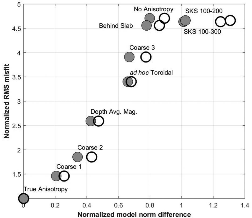
Figure 14. Normalized RMS misfit versus normalized norm difference for various models with respect to the model resulting from prescribing the “true anisotropy” field. The names of the approximate anisotropy field are indicated next to the corresponding symbols. Filled symbols correspond to calculations using the entire models, open symbol correspond to calculations that use only depths from 0 to 250 km.
