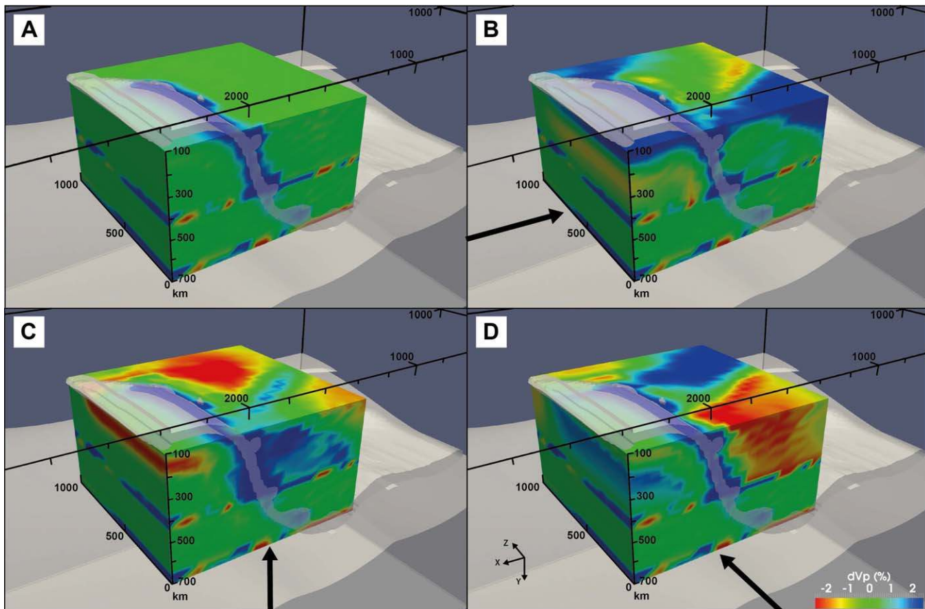
Figure 3. Isotropic and direction-dependent Vp anomalies for the “true” model. Views of dVp/Vp for the input model when considering isotropic velocities (a), and anisotropic velocities when the direction of propagation is East-West (b), vertical (c), and North-South (d). For clarity, the voxels corresponding to the slab are translucent. For similar figures showing dVs 1 /Vs 1 and Vp/Vs 1 ratio, the reader is referred to the supporting information.
