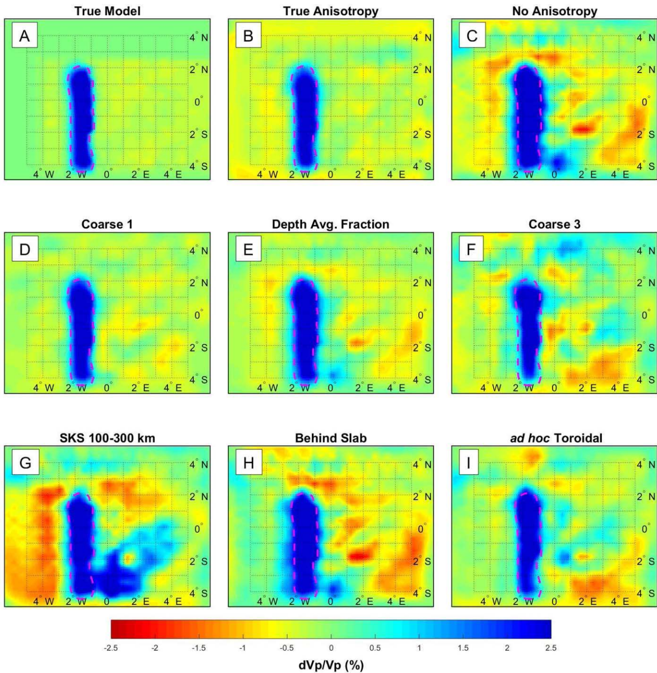
Figure 12. Results of inverting anisotropic delays while using different anisotropy fields as a priori constraints (b–i) and “true” model for comparison (a). For Figures 12b–12i, the name of the anisotropy field used in each case is indicated above each plot. The 1% isovelocity contours for the “true” model are shown as magenta-colored dashed lines for reference. All plots represent depth slices at 195 km. The severity of the artifacts varies according to the accuracy of the approximate anisotropy field used. For figures showing four depth slices and two cross sections for each of the models, the reader is referred to the supporting information.
