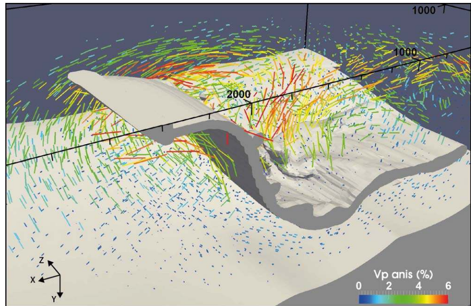
Figure 2. Vp anisotropy field for the “true” model. Light gray volumes represent areas of the model with viscosity above 9 \times 10^{22} Pa·s with the subducted slab being clearly identifiable. Colored bars represent the anisotropy developed in the polycrystalline aggregates. Bar orientation indicates the fast Vp propagation direction, and bar length and color indicate magnitude of anisotropy.
