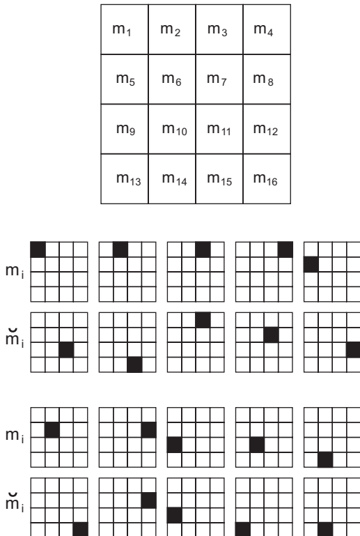
Fig. 6. Left: iconic depiction of the relations according to the arrangement of relations in Fig. 4; right: table of converse relations (note that \tilde{m}_i = m_i ); each relation that holds is printed in black; each converse relation is unambiguous.
