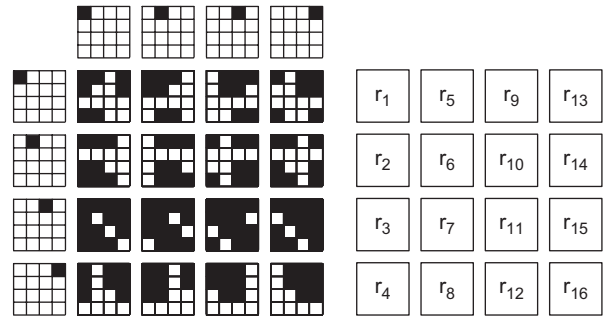
Fig. 7. Non-atomic core compositions r_1 to r_{16} . It holds that r_5 = r_1^{\rightarrow} , r_9 = r_5^{\rightarrow} , r_{13} = r_9^{\rightarrow} , r_1 = r_{13}^{\rightarrow} , r_6 = r_2^{\rightarrow} , etc. Consequently, only r_1 to r_4 have to be explicitly defined.
