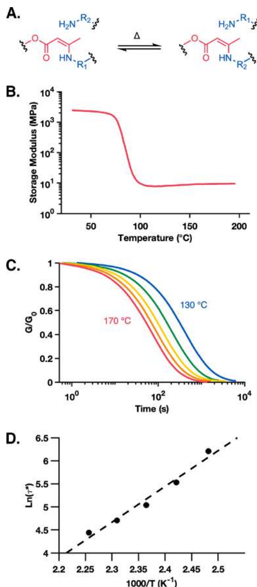
Figure 4. (A) Structure of cross-linked vinylogous urethanes that relax stress through an associative reaction and demonstrate the characteristic properties of vitrimer. (B) A DMTA trace exhibits a constant storage modulus above T_g . (C) Normalized stress relaxation analysis at temperatures between 130 and 170 °C. (D) Arrhenius plot of the characteristic relaxation time ( \tau^* ) against inverse temperature.
