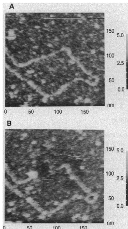
Fig. 5. Dissection of plasmids with the AFM. (A) and (B) are BlueScript II plasmid-imaged in propanol before (A) and after (B) scanning an area of ~30 nm by 30 nm at high force. Note upper region of plasmid that has been dissected away in (B). Plasmid width in (A) is 4 to 5 nm; in (B), after the high-force scan, evidence of a double tip is seen. Image sizes are 200 nm by 200 nm. The images have been processed only by flattening to remove background slope.
