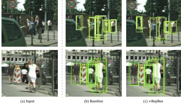
Figure 7. Visualized comparison of predicted bounding boxes before NMS of baseline and RepBox. In the results of RepBox, there are fewer predictions lying in between two adjacent ground-truths, which is desirable in crowd scenes. More examples are shown in supplementary material.
