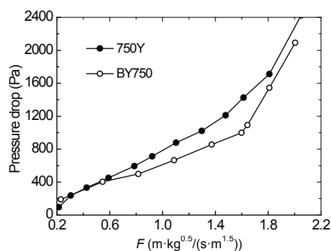
Fig. 9 Pressure drop performance of BY750 series structured packing developed by Peiyang
