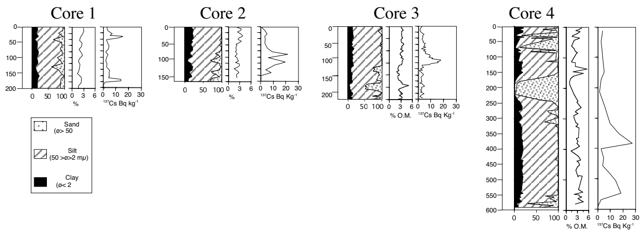
Fig. 3. Distribution of grain size and organic matter percentages and 137 Cs activity curves in the sediments of the four cores in the reservoir.
