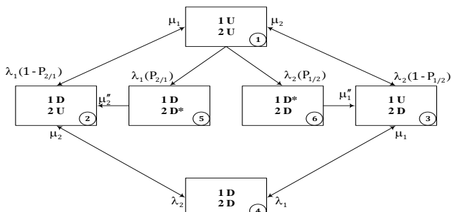
Fig. 1. State transition diagram of a 2-component system considering independent, dependent mode and dependent mode initiating outages
