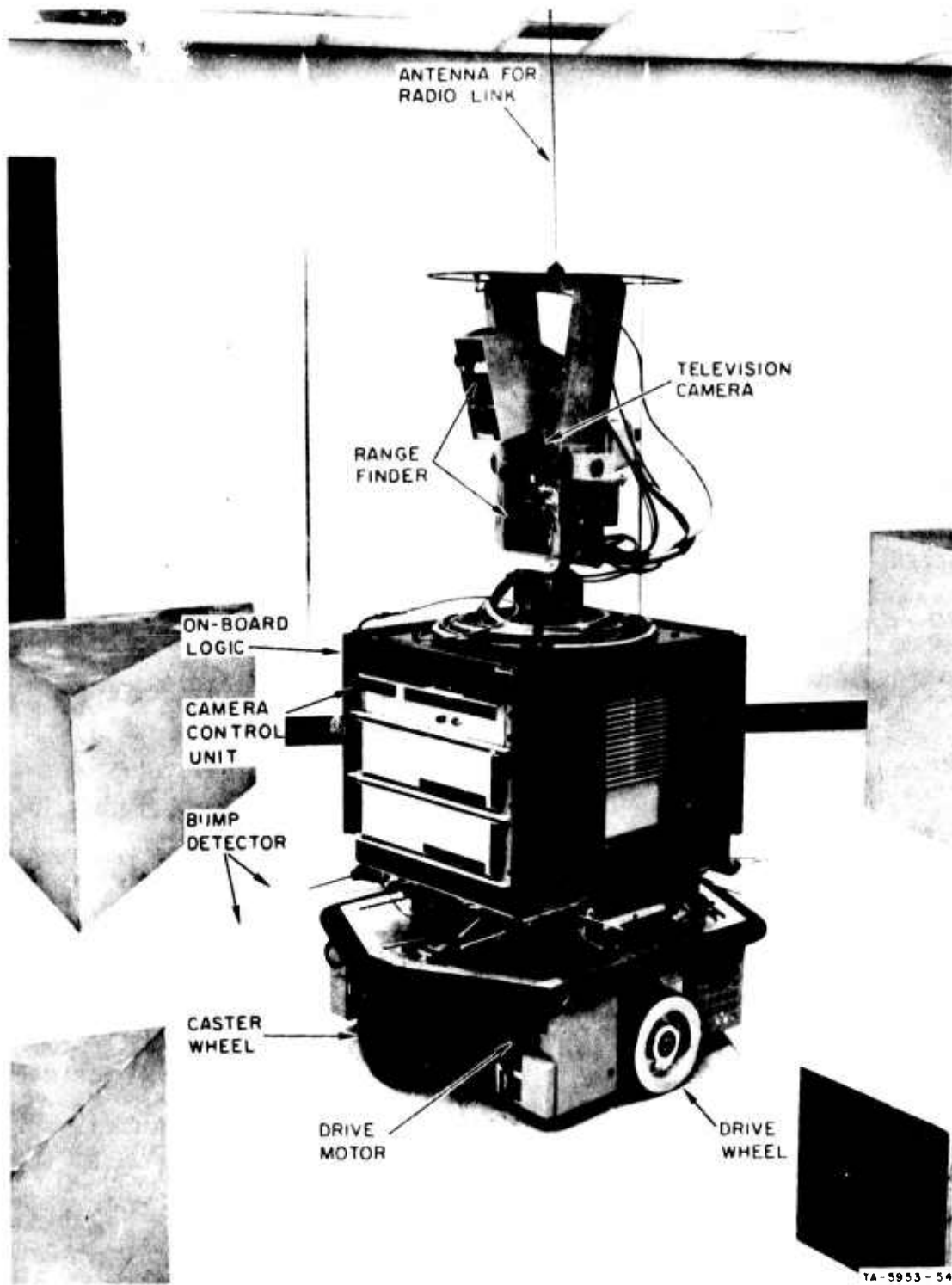
Figure 1. The Robot Vehicle
