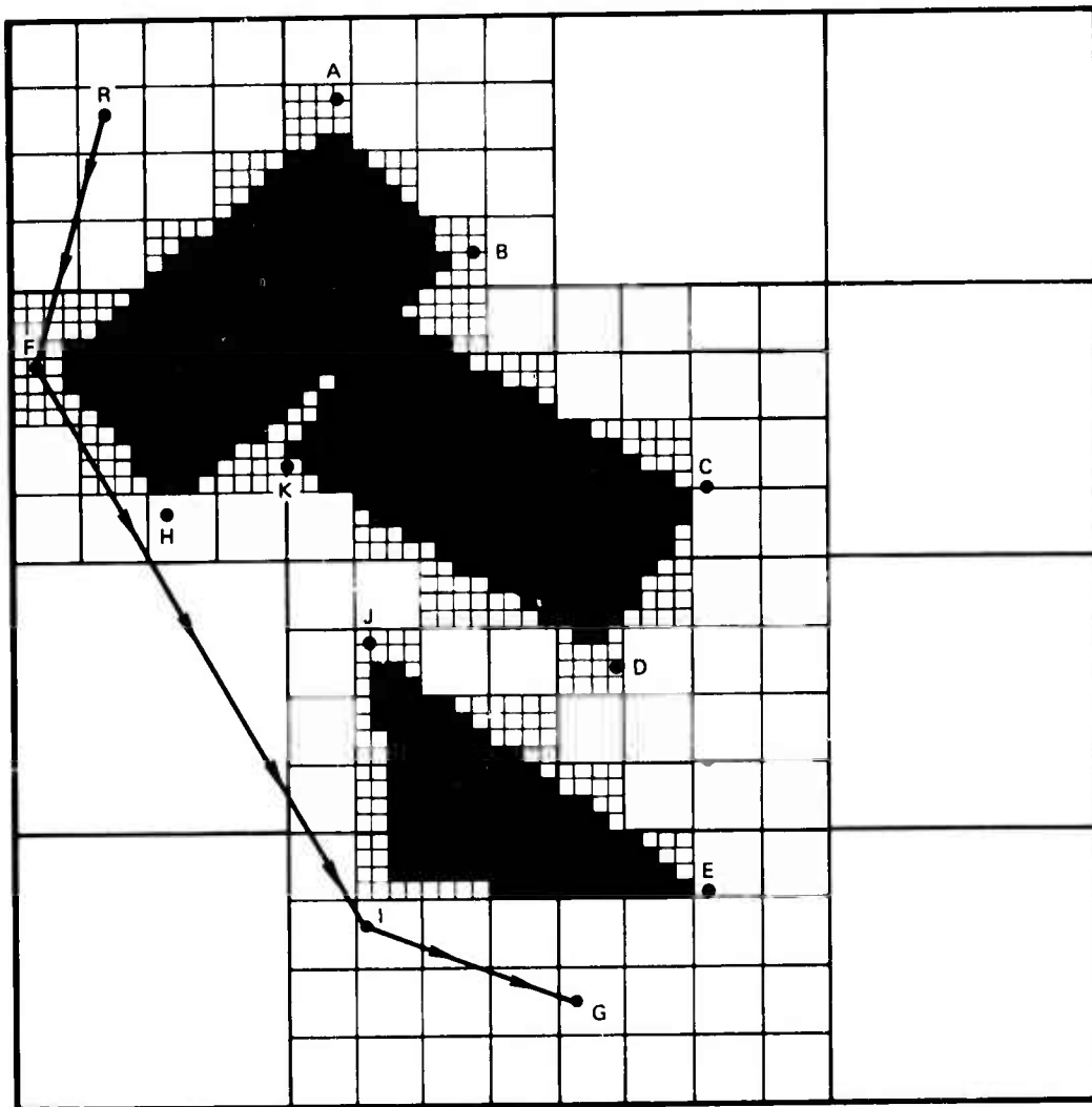
Figure 2. A Grid Model of a Room With Three Objects
