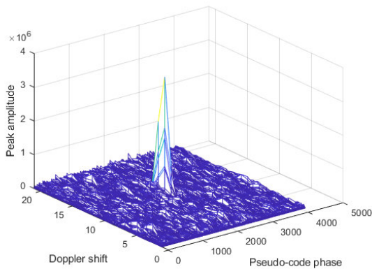
FIGURE 2. The authentic satellite signal in the acquisition phase.
