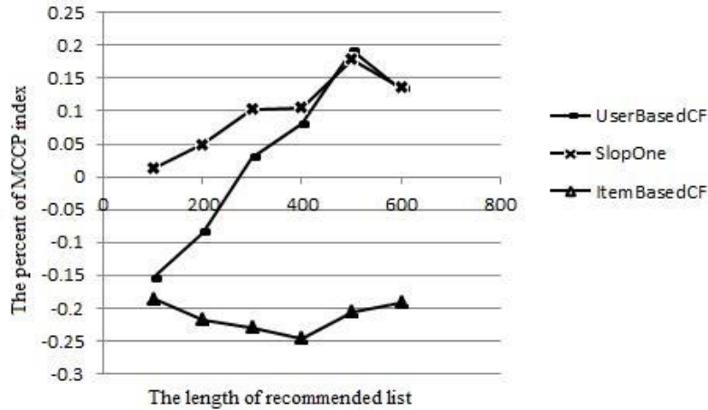
Figure 2. The Accuracy Metric of Recommendation Algorithm
