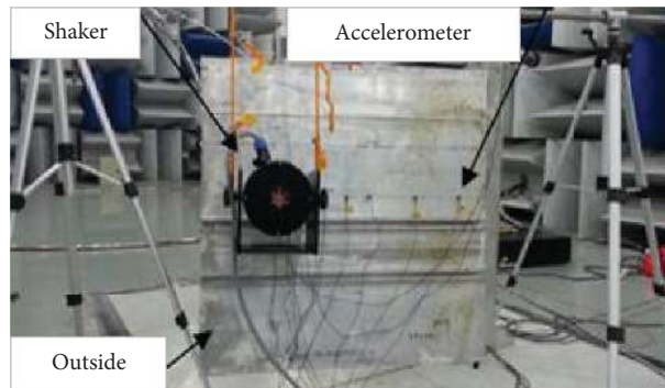
FIGURE 10: ESEA test process of incentive point B.
