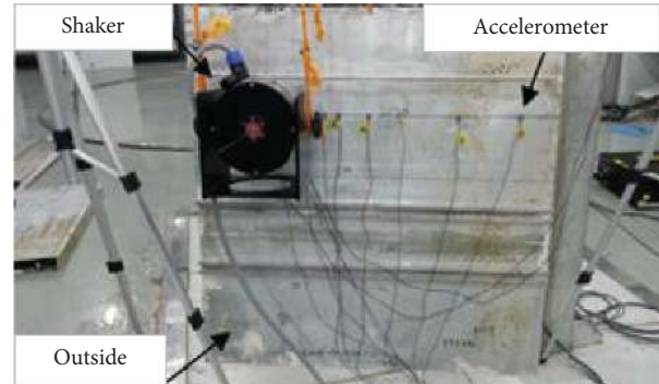
FIGURE 9: ESEA test process of excitation point A.
