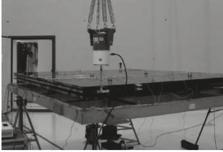
FIGURE 3: PIM method test input power.
