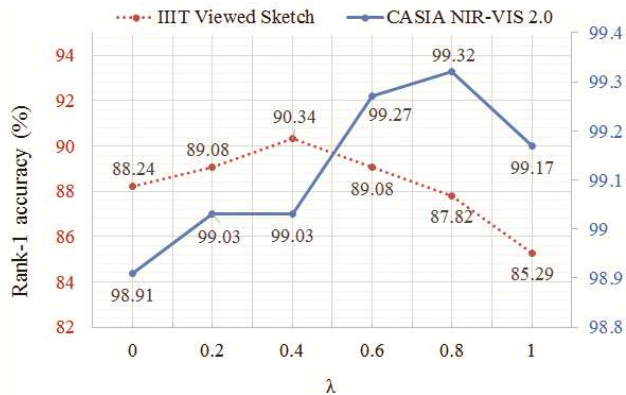
Figure 5: Rank-1 accuracy on IIIT-D Viewed Sketch and CASIA NIR-VIS 2.0 with varied \lambda .
