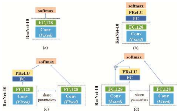
Figure 3: The architectures of four baseline models. (a) and (b) are single-branch while (c) and (d) are two-branch. (d) includes our default RC module.
