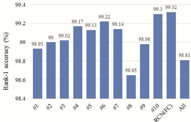
Figure 4: Evaluation of RC position on CASIA NIR-VIS 2.0. # k ( k = 1, 2, ..., 10) means we add RC module to the k -th convolutional layer. ‘All’ means adding RC module to all layers.
