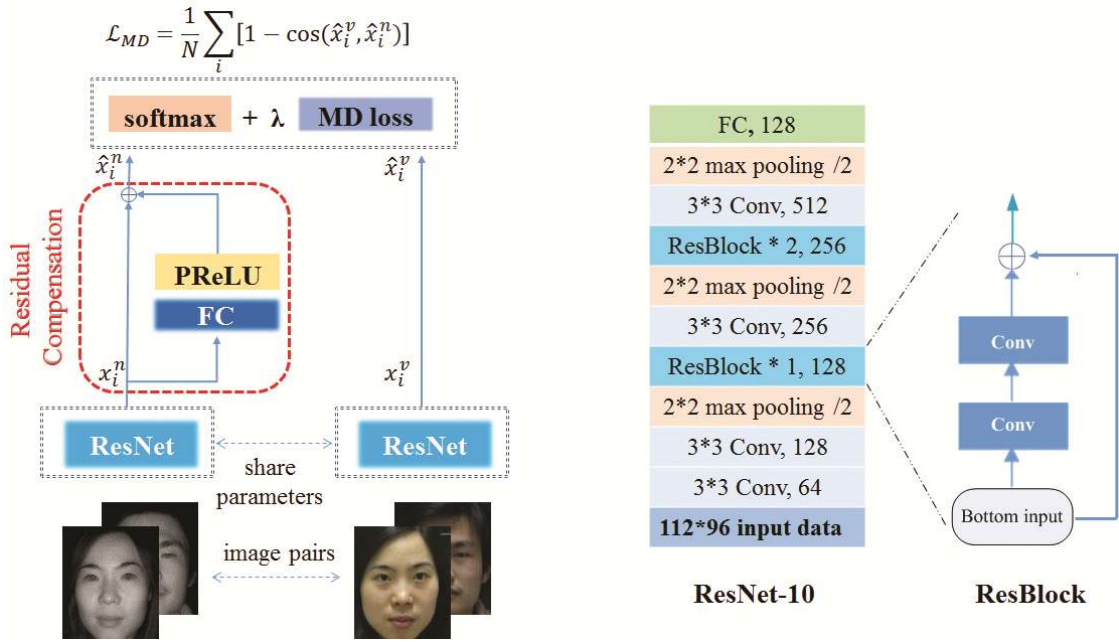
Figure 1: The pipeline of the our RCN. Left: the two-branch architecture of RCN. Right: the backbone model of RCN.
