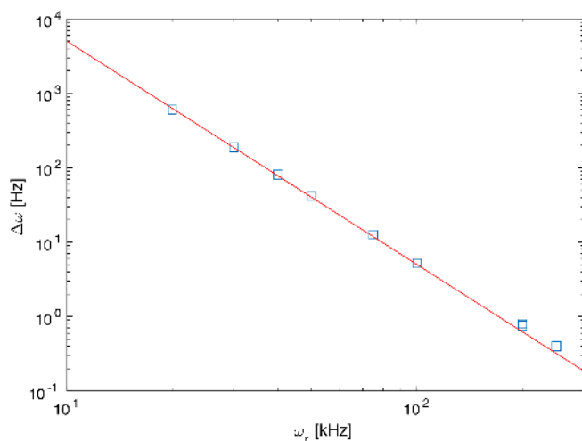
Figure 3. Difference in breadth of the simulated spectra between the third-order and exact effective Hamiltonians as a function of the spinning frequency. The red line has a slope of -3 corresponding to a \omega_r^{-3} dependence of the difference. This is the expected slope for a contribution by a fourth-order effective Hamiltonian.
