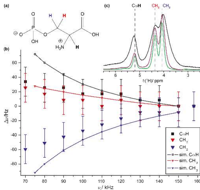
Figure 8. MAS dependence of 1 H line positions in ortho-phospho-L-serine (for the chemical structure, see panel a). (b) The filled symbols indicate experimental data with a constant error of 20 Hz. The two CH 2 protons are shown in red (high ppm peak) and blue (low ppm peak); the C \alpha H proton is shown in black. The simulations were based on a three-spin system with r_{12} = 1.60 Å, r_{23} = r_{13} = 2.35 Å, and \theta(1, 2, 3) = \theta(2, 1, 3) = 70^\circ . Three 1 H spectra recorded with MAS frequencies of 70 kHz (black), 120 kHz (purple), and 158 kHz (green) are shown in panel (c). The dashed lines indicate the isotropic 1 H chemical shift at 158 kHz MAS. The experiments were performed at a static magnetic field of 20 T.
