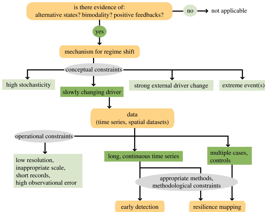
Figure 3. A map of conceptual, operational and methodological considerations when applying CSD indicators for the detection of critical transitions and resilience mapping. Light green colours indicate cases where early detection is less likely. (Online version in colour.)
