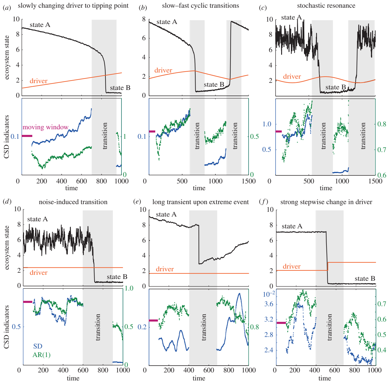
Figure 1. (a–f) Six different mechanisms can lead to regime shifts with or without crossing a tipping point. Based on the mechanism, early warnings may or may not indicate the approaching shift. Black lines indicate time series of the ecosystem state, red lines time series of underlying environmental conditions. Standard deviation (s.d., blue) and autocorrelation at-lag-1 (AR1, green) were estimated from the detrended time series of ecosystem state within moving windows up to the regime shift (details in the electronic supplementary material). (Online version in colour.)
