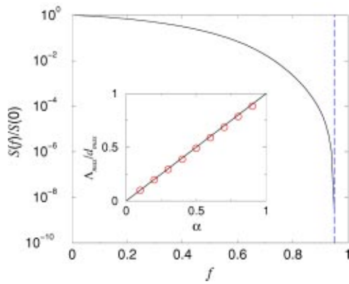
FIG. 1. Size of the giant component for a graph with p_d = cd^{-3.5} ( 2 \leq d \leq d_{max} , d_{max} = 100 ) and degree correlations p(d'|d) = \alpha \delta_{dd'} + (1-\alpha)q_{d'} with \alpha , as computed from Eq. (4). The dashed line marks the percolation threshold obtained using perturbation theory [Eq. (18)]. The inset shows the largest eigenvalue relative to d_{max} as a function of \alpha . The points were computed numerically and the line is the perturbation theory dependency \Lambda_{max}/d_{max} = \alpha .
