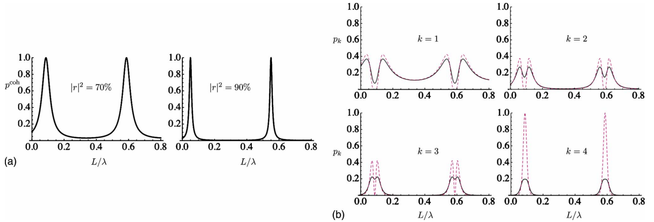
FIG. 3. (Color online) (a) shows the classical normalized transmission function as a result of Eq. (5) displayed for a reflectivity of |r|^2=70\% (LHS) and |r|^2=90\% (RHS) of the FPI-mirrors. Note that the transmission peaks become narrower and the maxima slightly shifted to the left as the reflectivity increases. Also the minima go to zero for 90% reflectivity whereas they do not reach zero for lower reflectivities. (b) shows the probabilities of detecting k photons, p_k^{\text{coh}} for a single-mode coherent input state |\alpha\rangle with mean photon number \bar{n}=|\alpha|^2=4 incident on the FPI and a photon-number resolving measurement displaying k=1, \dots, 4 (solid lines). The dashed lines shows the transmission probabilities p_k^{\text{F}} for a single-mode photon-number state |4\rangle . We observe that the Fock states (dashed lines) show transmission peaks that are sharper in general. This effect is equivalent to operating at a larger reflectivity of the mirrors, which is demonstrated in (a) for the classical curves. A major difference appears for k=4 where the transmission maxima reach one for the Fock state, whereas the coherent state stays low. Here and in the following, we choose a reflectivity of 70% as the important features are more pronounced than for larger reflectivities.
