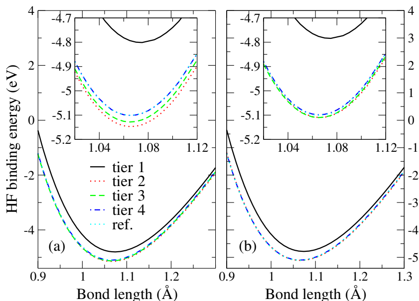
Figure 8. HF binding energy of N_2 as a function of the bond length for different levels of NAO basis sets (from tier 1 to tier 4). The reference curve (denoted as ‘ref’) is obtained with NWChem and a Gaussian cc-pV6Z basis. (a) Results without BSSE corrections; (b) BSSE-corrected results. The insets magnify the equilibrium region.
