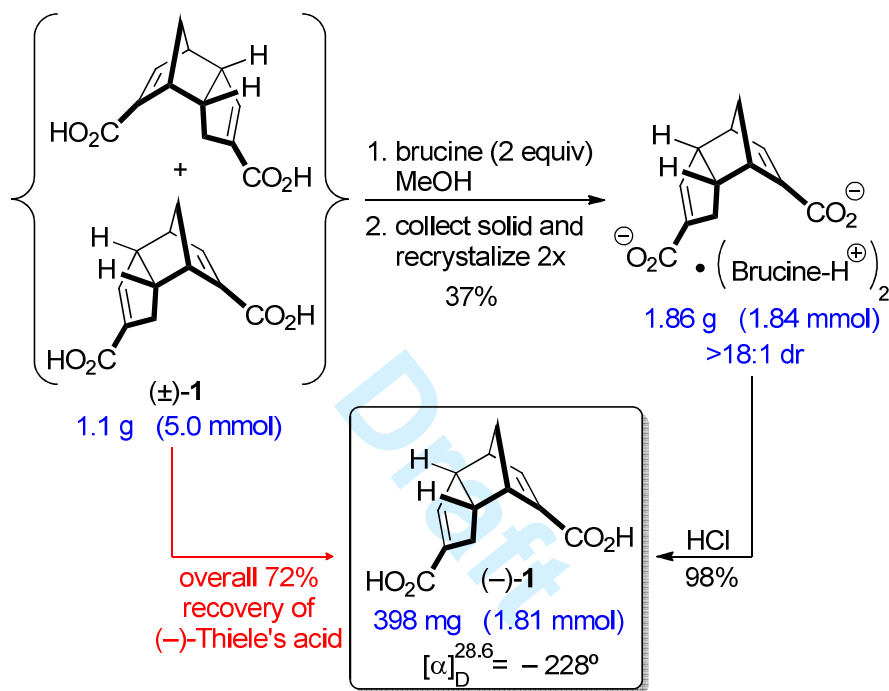
Scheme 3. Resolution of Thiele's acid.
