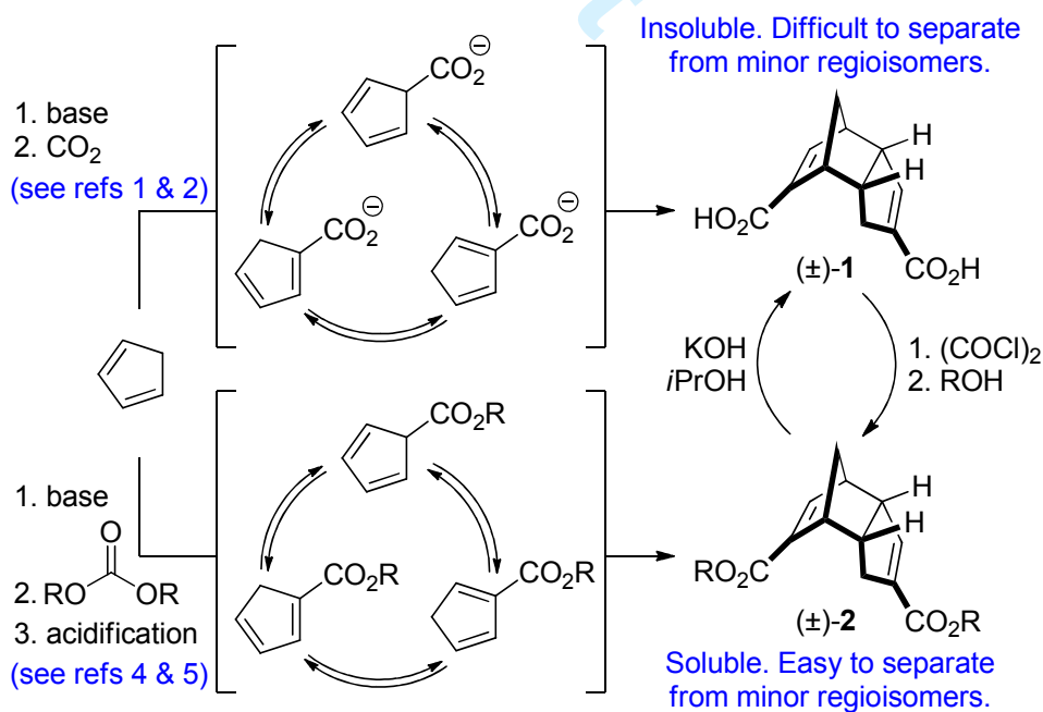
Scheme 1. Synthetic approaches to Thiele's acid and esters.
