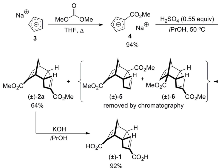
Scheme 2. Synthesis of racemic Thiele's acid.
