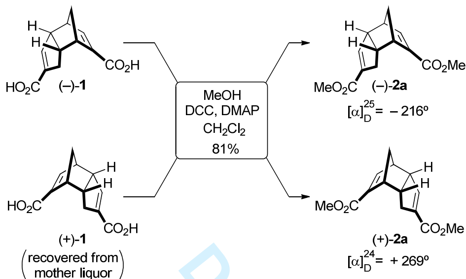
Scheme 4. Esterification of resolved Thiele's acids.
