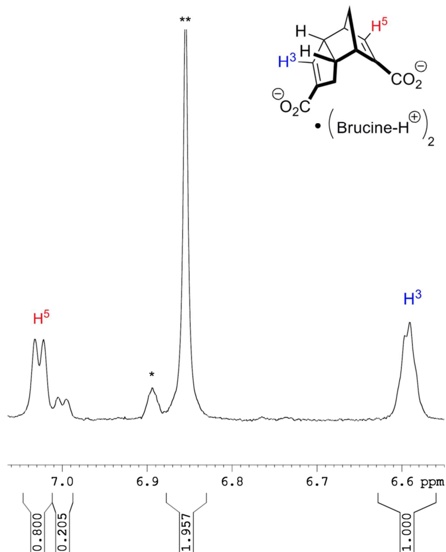
Figure 2. ^1\text{H} NMR spectrum of the bis-brucine salt of 1 after the first recrystallization from methanol, recorded in 8.3:1 \text{C}_6\text{D}_6:\text{CDCl}_3 . Signals corresponding to the two vinyl C-H protons are labeled. The peaks indicated by the single and double asterisks correspond to a ^{13}\text{C} satellite from benzene and an aromatic C-H from brucine, respectively.
