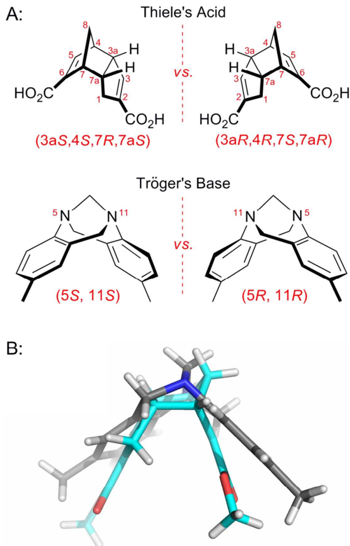
Figure 1. Comparison of Thiele's acid to Tröger's base. A: Structures and stereochemical assignment for each compound. B: Overlay of Tröger's base (gray) and Thiele's acid methyl ester (cyan), revealing a narrower cleft angle for the latter compound.
