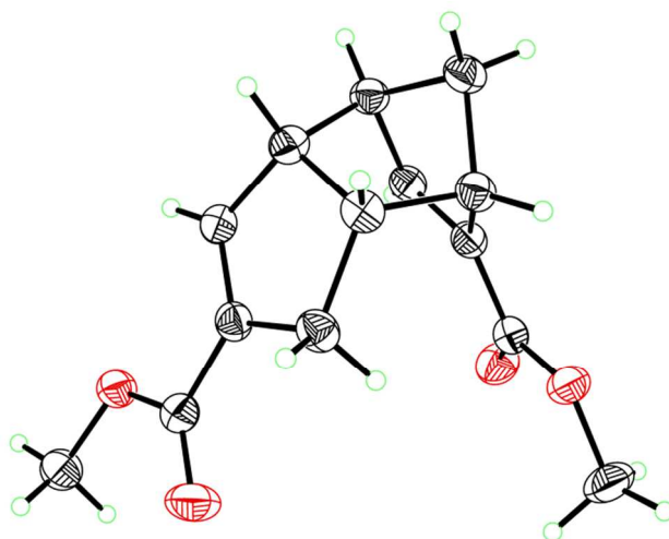
Figure 3. X-ray structure for (-)-2a . Thermal ellipsoids are shown at 50% probability.
