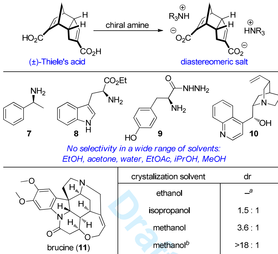
Chart 1. Formation of Diastereomeric Salts from Thiele's Acid.
